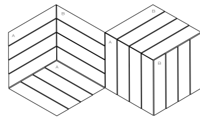
A & B Cube Installation
