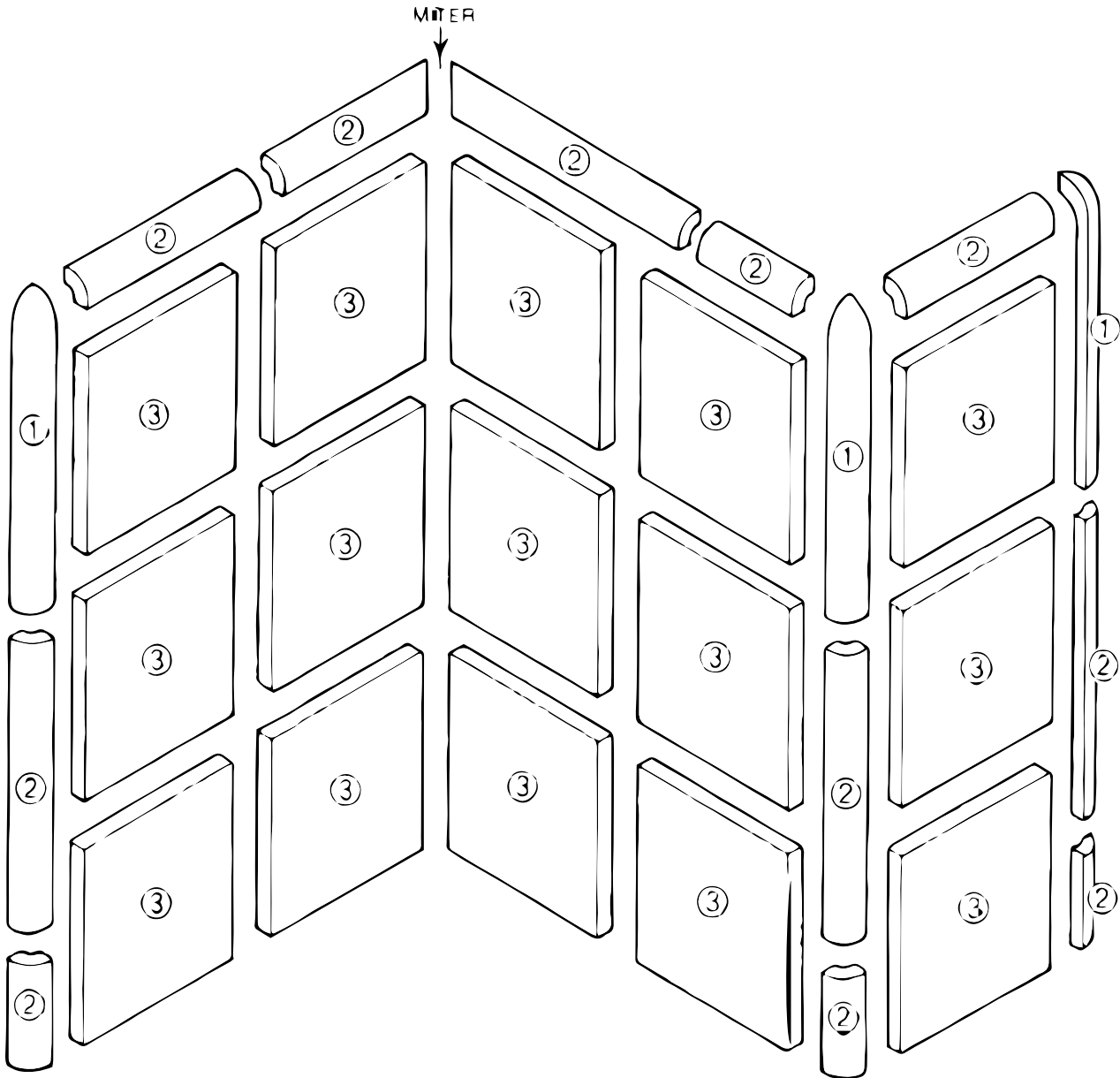
4 1/4"x4 1/4" Conventional Square in Corners
